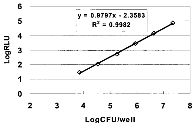
Figure 1 Correlation of luminescent signal (log RLU) and viable counts (log CFU) of bioluminescent S. enteritidis strain in a 96-well microplate at room temperature. Fivefold serial dilutions of the culture were prepared in triplicate in LB broth with 200 \mu l per well. The total RLU in each well was measured by a microplate luminometer. Samples from each well were plated, and CFU/well was determined.
