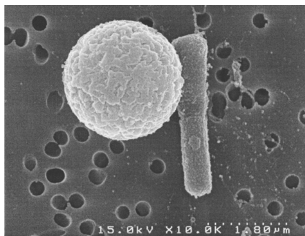
Figure 3 Scanning electron micrograph of an S. enteritidis cell captured by the constructed biosorbent.
